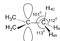
Scheme 2. Bond angle evidence for \text{C}-\text{H}(4\text{C}) bond hyperconjugation in the C4 methyl group.
